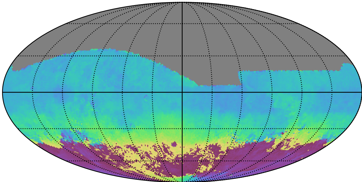
too_10_4v3.4_10yrs All sky g band: AngleMean rotSkyPos
