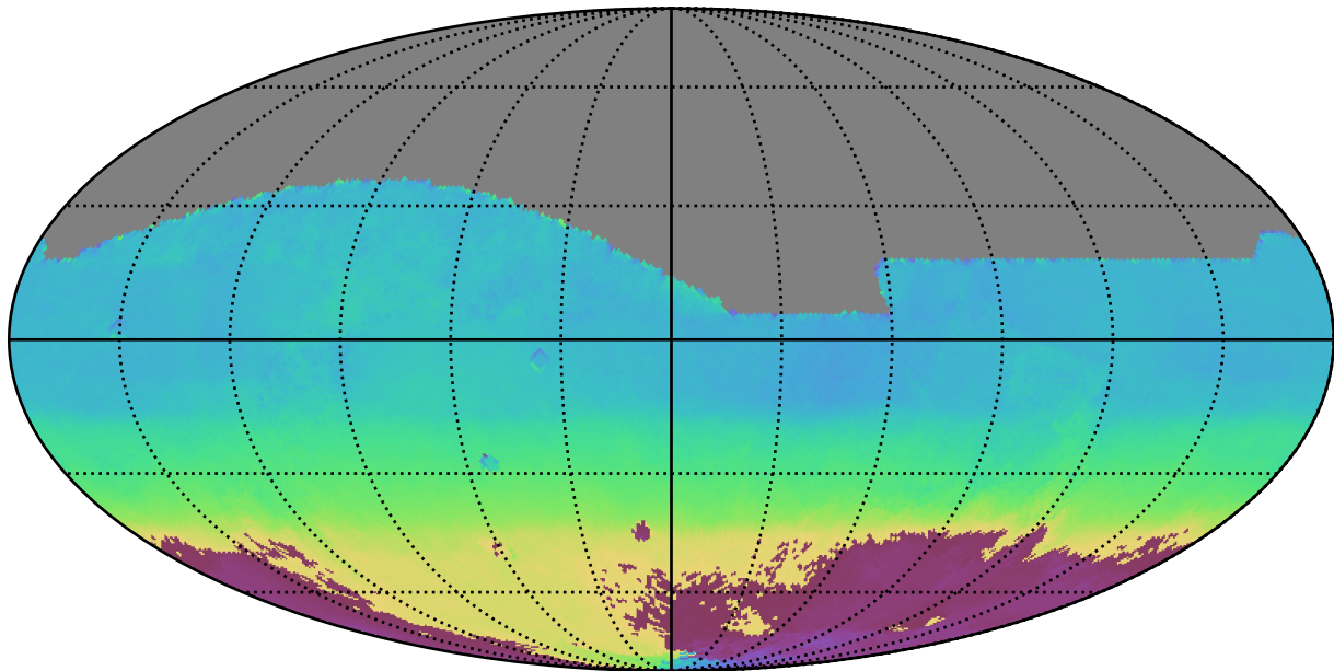
too_10_4v3.4_10yrs All sky all bands: AngleMean rotSkyPos
