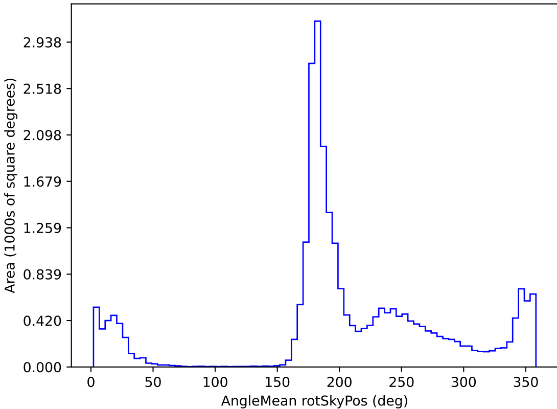
too_10_4v3.4_10yrs All sky all bands: AngleMean rotSkyPos
