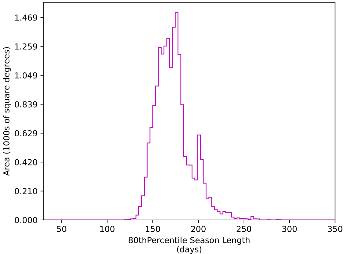
too_10_4v3.4_10yrs WFD z band: 80thPercentile Season Length
