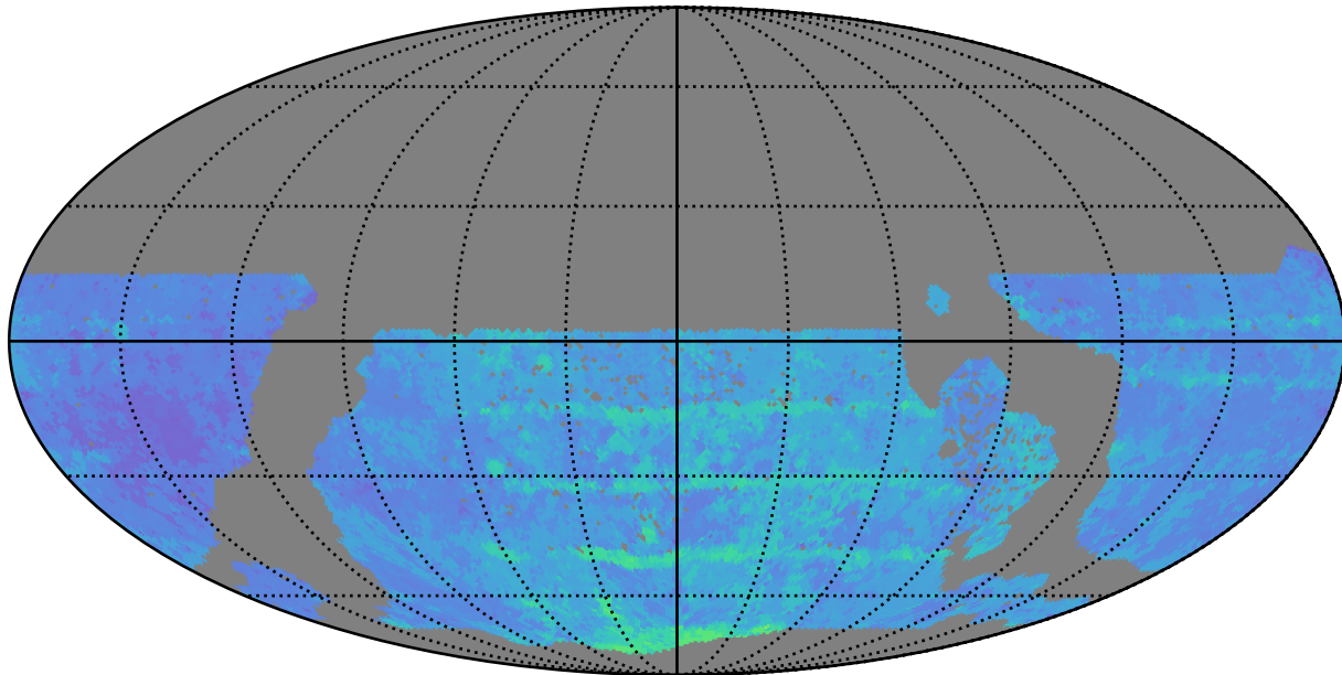
too_10_4v3.4_10yrs WFD y band: 80thPercentile Season Length
