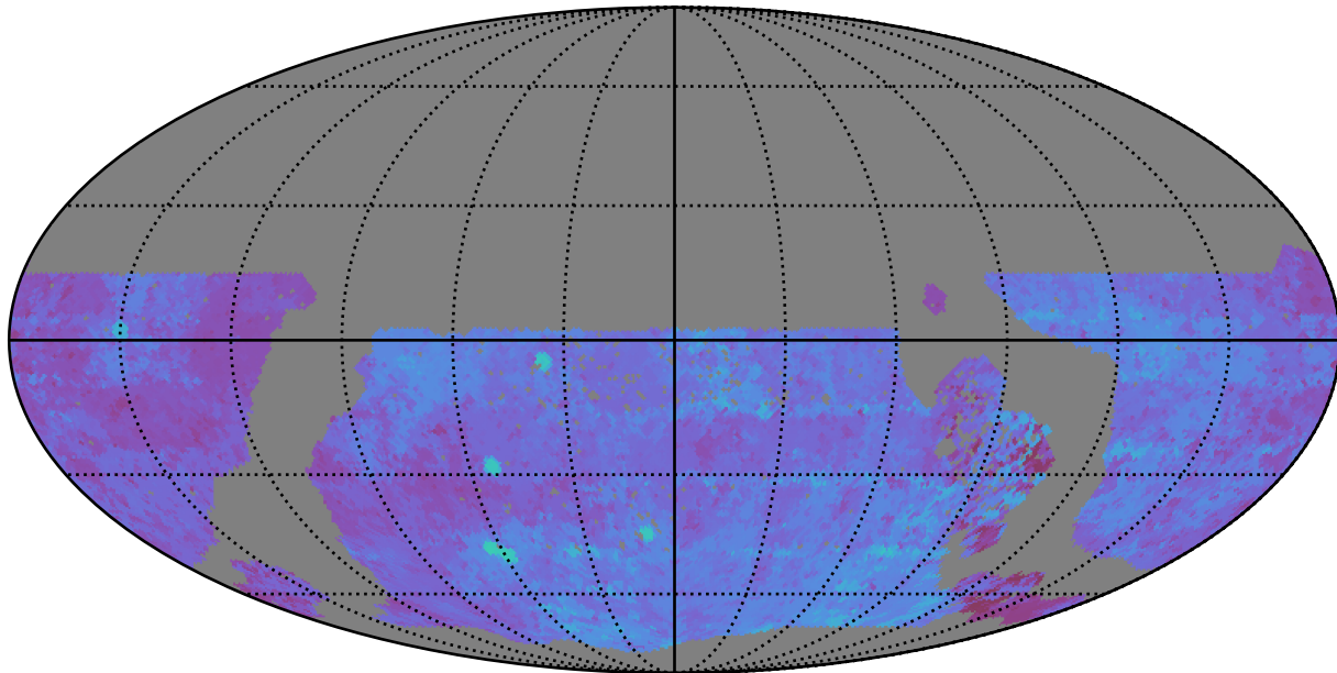
too_10_4v3.4_10yrs WFD u band: 80thPercentile Season Length
