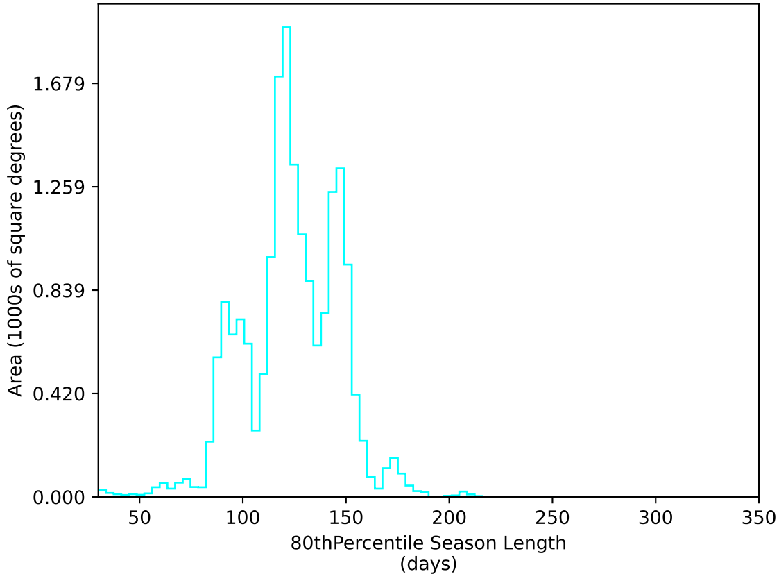
too_10_4v3.4_10yrs WFD u band: 80thPercentile Season Length
