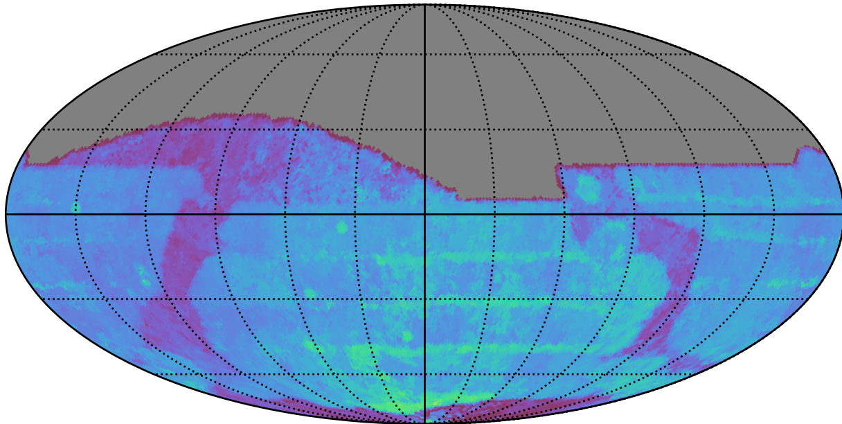
too_10_4v3.4_10yrs All sky z band: 80thPercentile Season Length
