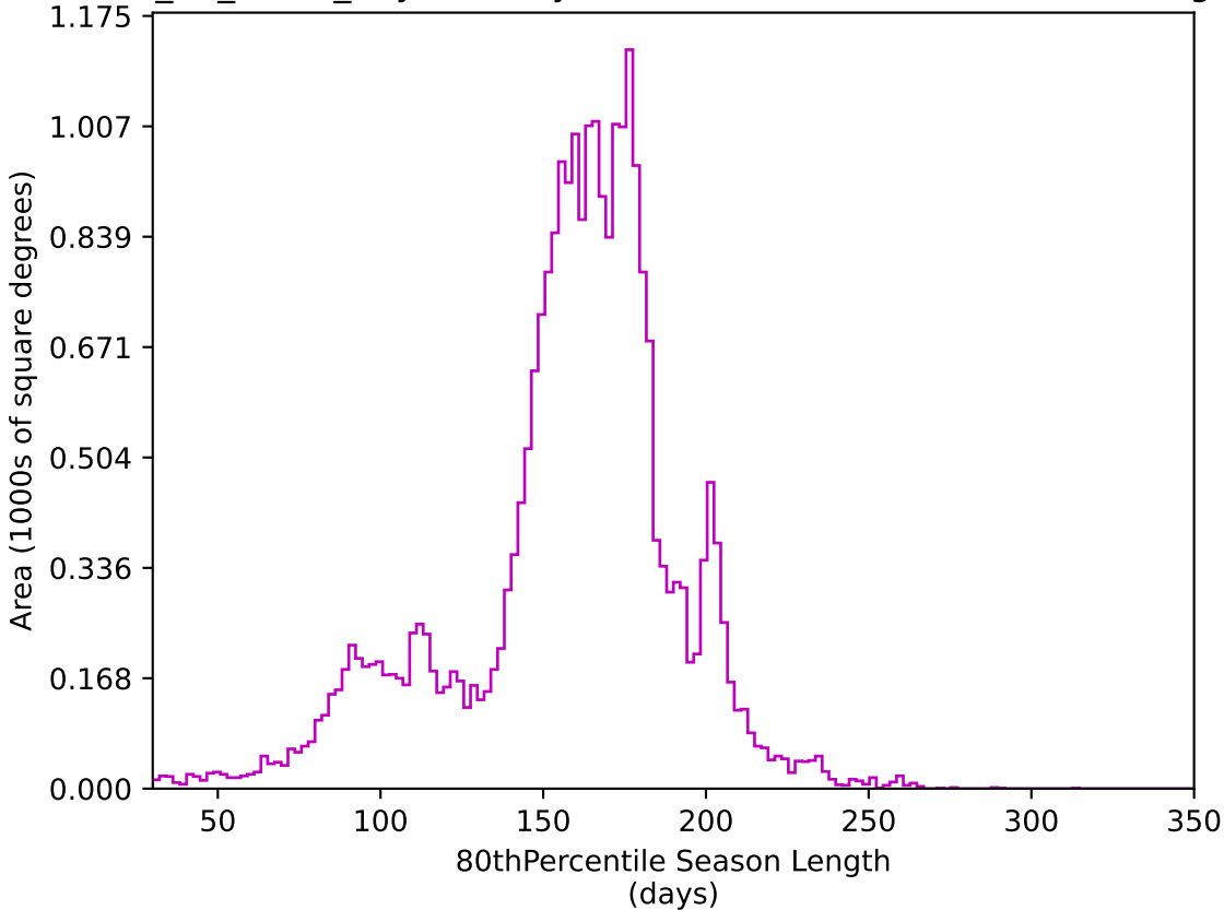
too_10_4v3.4_10yrs All sky z band: 80thPercentile Season Length
