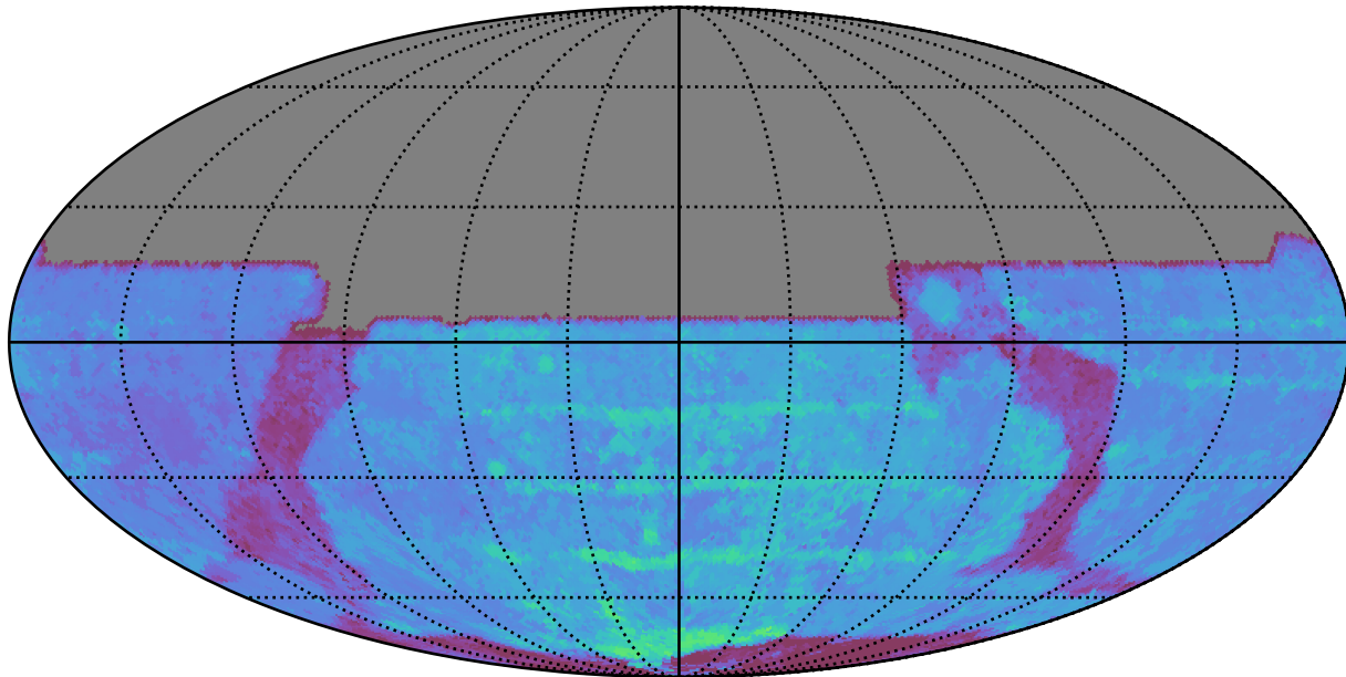
too_10_4v3.4_10yrs All sky y band: 80thPercentile Season Length
