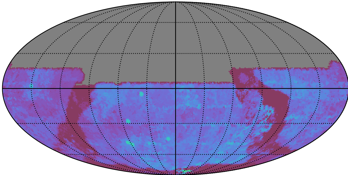
too_10_4v3.4_10yrs All sky u band: 80thPercentile Season Length
