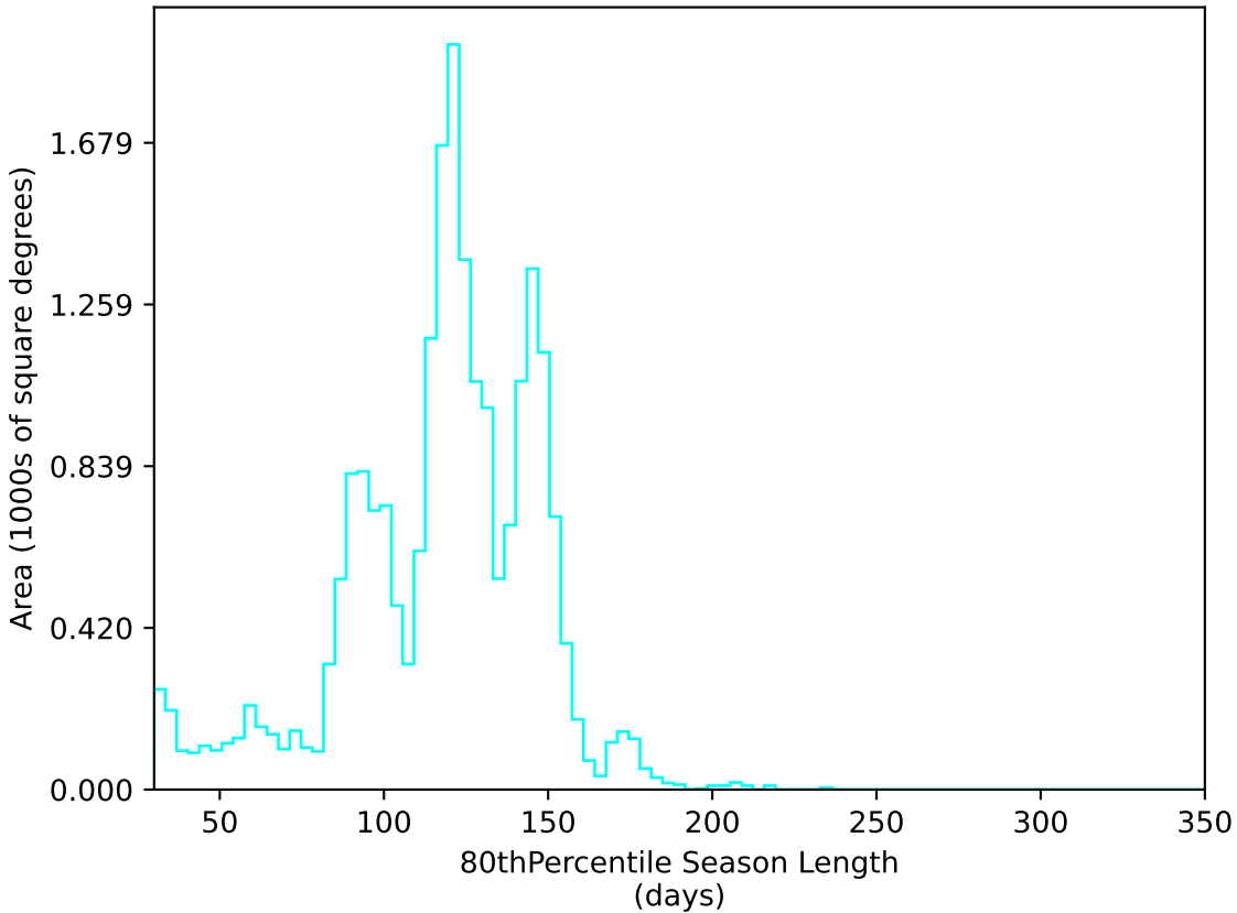
too_10_4v3.4_10yrs All sky u band: 80thPercentile Season Length
