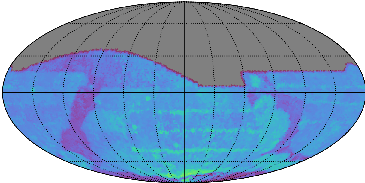
too_10_4v3.4_10yrs All sky i band: 80thPercentile Season Length
