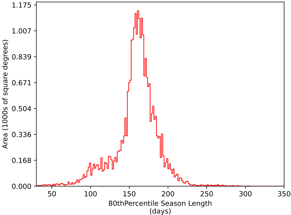
too_10_4v3.4_10yrs All sky i band: 80thPercentile Season Length
