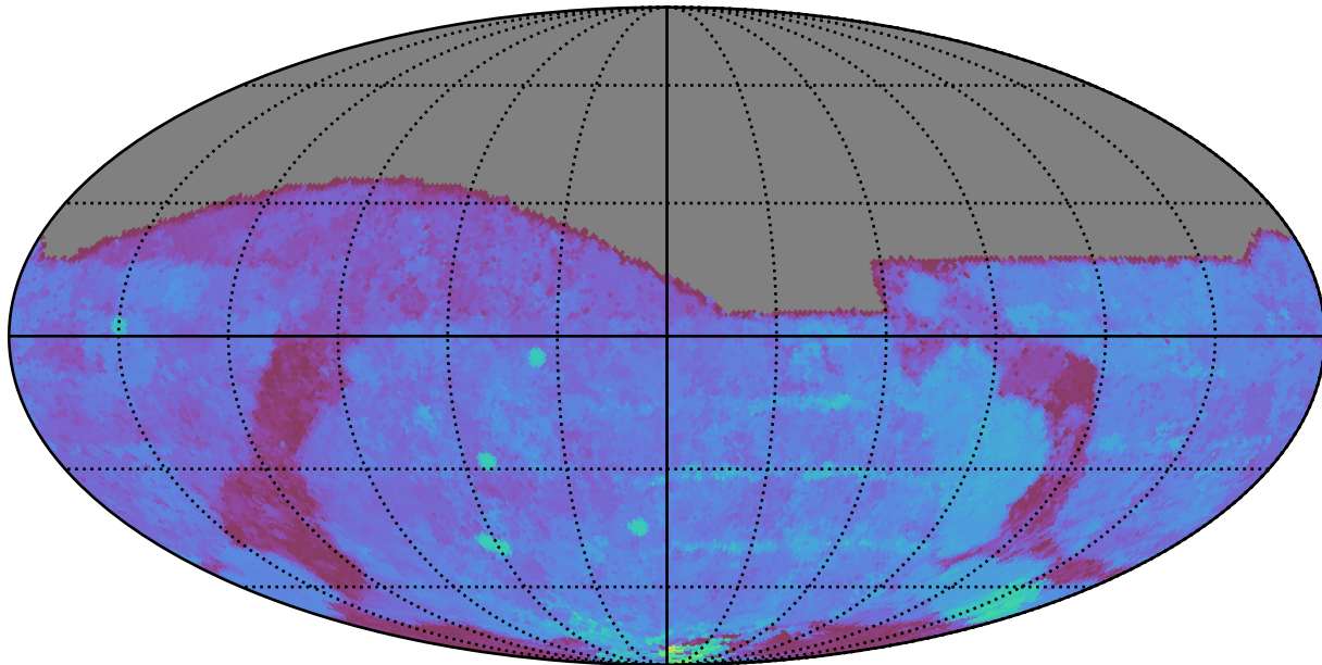
too_10_4v3.4_10yrs All sky g band: 80thPercentile Season Length
