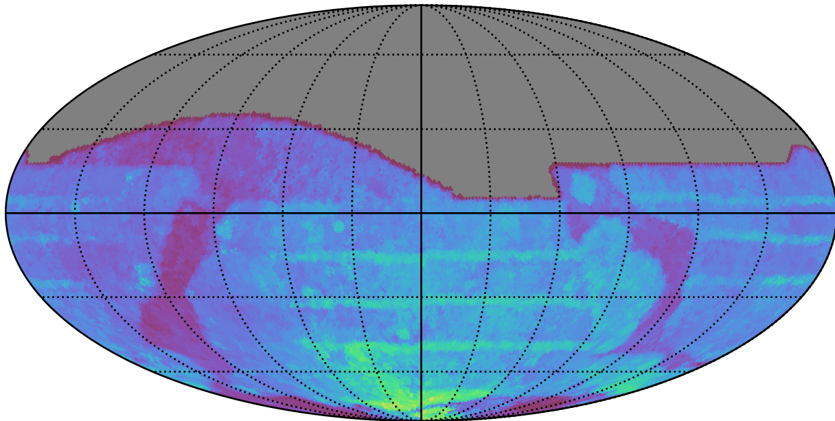
too_10_4v3.4_10yrs All sky all bands: 80thPercentile Season Length
