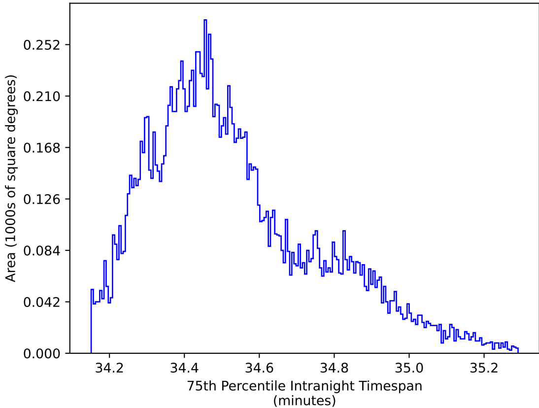
too_10_4v3.4_10yrs WFD zy bands: 75th Percentile Intranight Timespan
