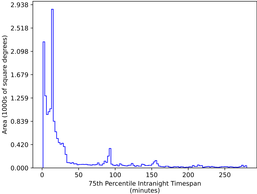
too_10_4v3.4_10yrs WFD r band: 75th Percentile Intranight Timespan
