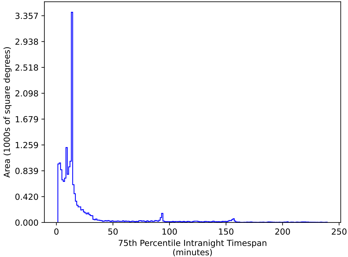
too_10_4v3.4_10yrs WFD i band: 75th Percentile Intranight Timespan
