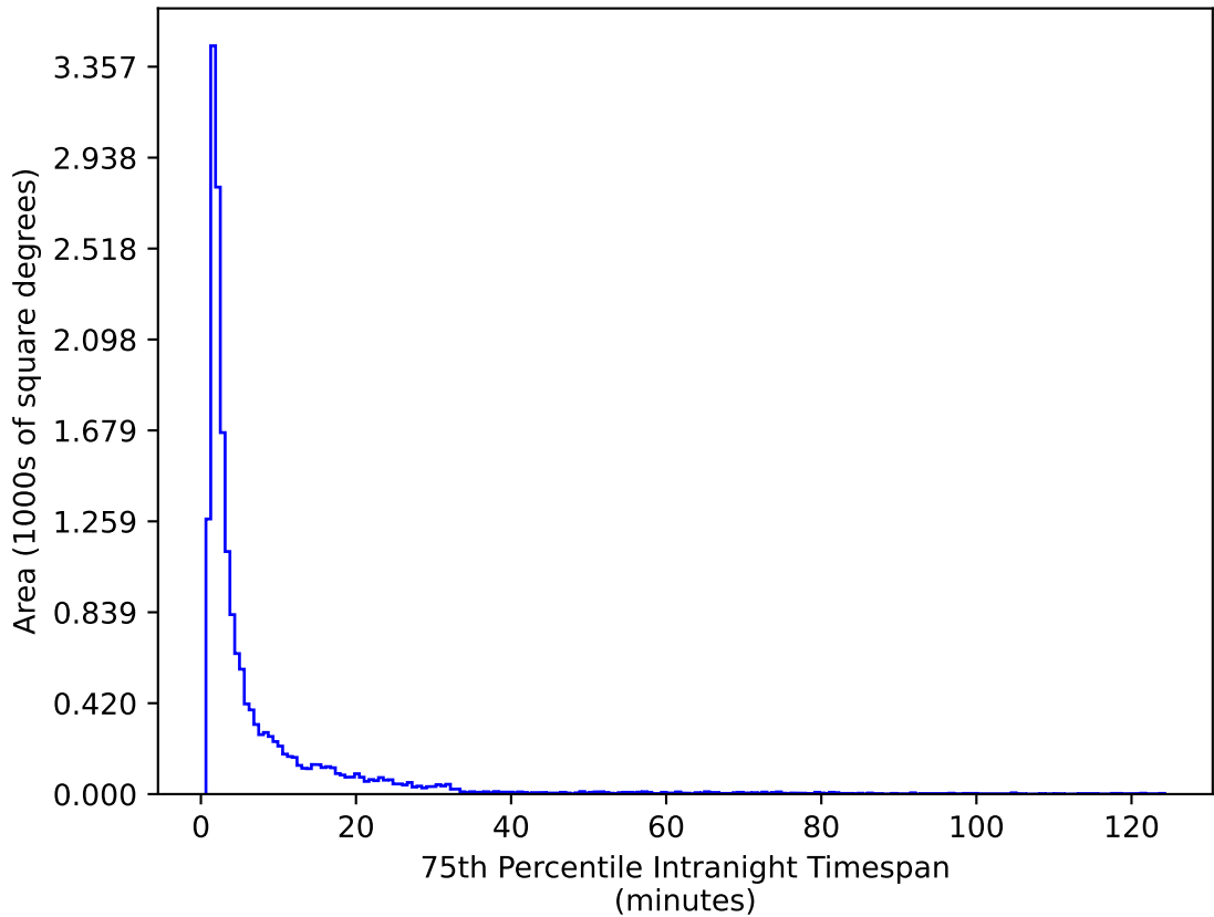
too_10_4v3.4_10yrs WFD g band: 75th Percentile Intranight Timespan
