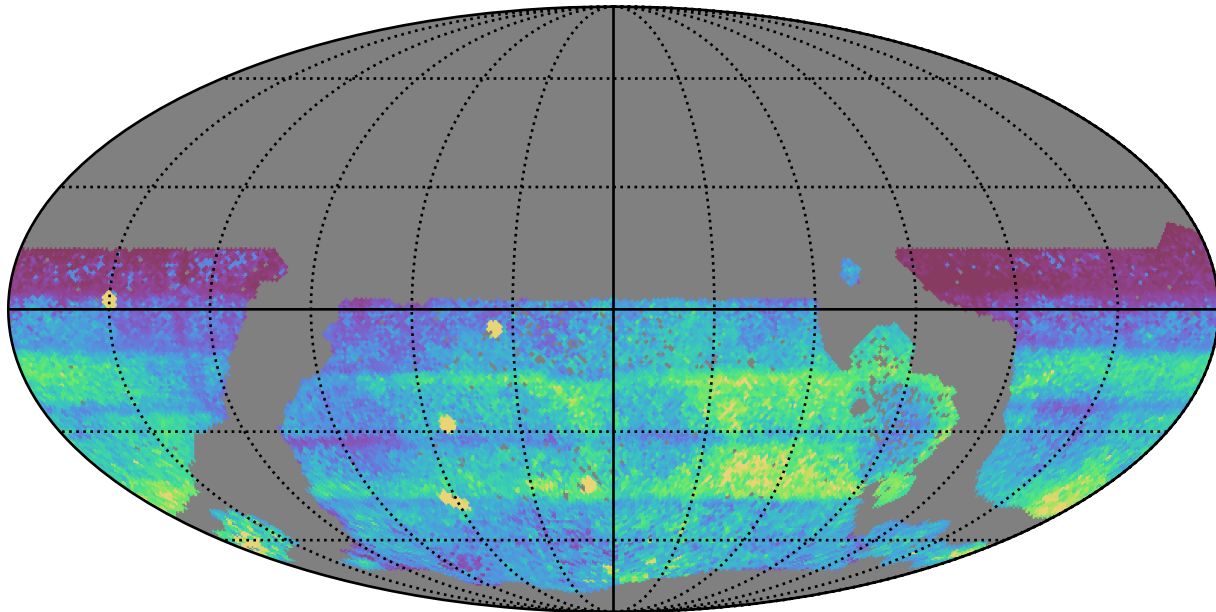
too_10_4v3.4_10yrs WFD: 75th Percentile Intranight Timespan
