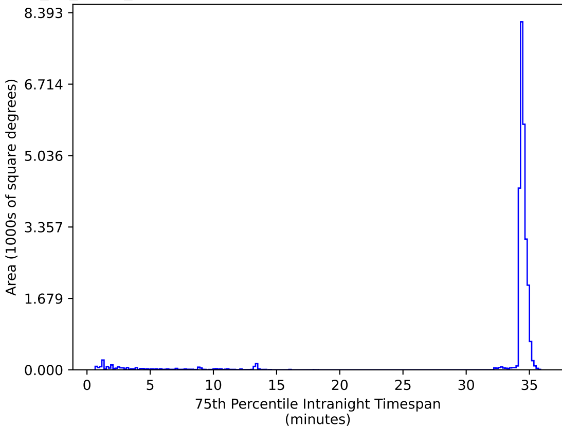
too_10_4v3.4_10yrs All sky zy bands: 75th Percentile Intranight Timespan
