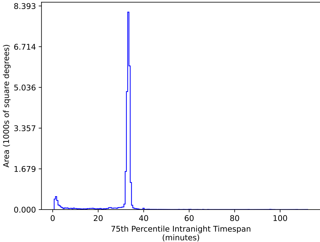
too_10_4v3.4_10yrs All sky ug bands: 75th Percentile Intranight Timespan
