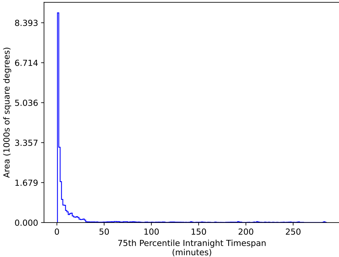
too_10_4v3.4_10yrs All sky u band: 75th Percentile Intranight Timespan
