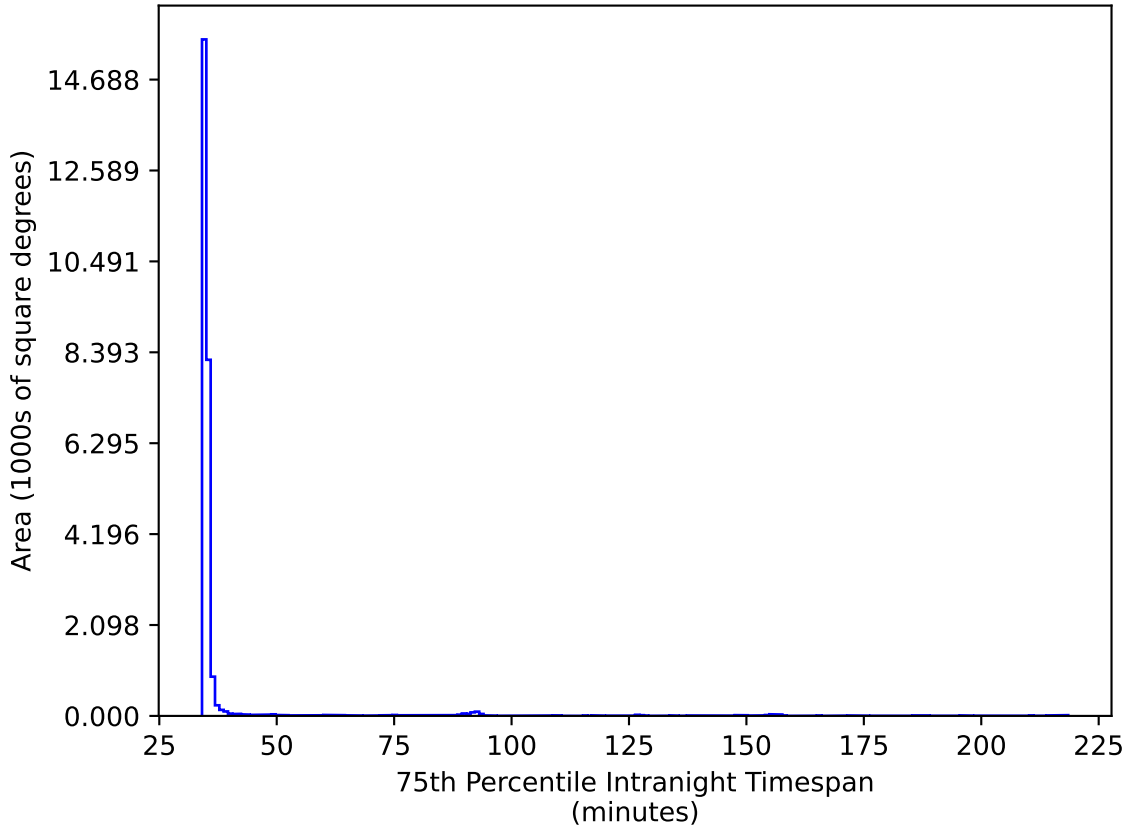
too_10_4v3.4_10yrs All sky ri bands: 75th Percentile Intranight Timespan
