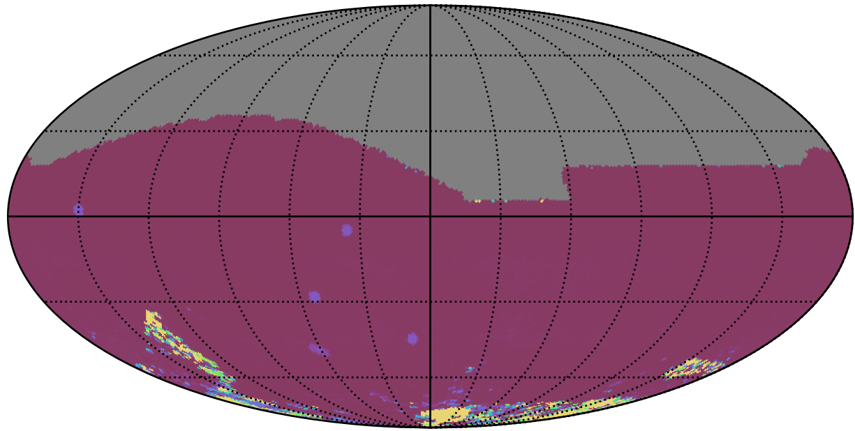
too_10_4v3.4_10yrs All sky iz bands: 75th Percentile Intranight Timespan
