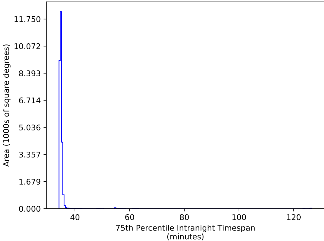
too_10_4v3.4_10yrs All sky iz bands: 75th Percentile Intranight Timespan
