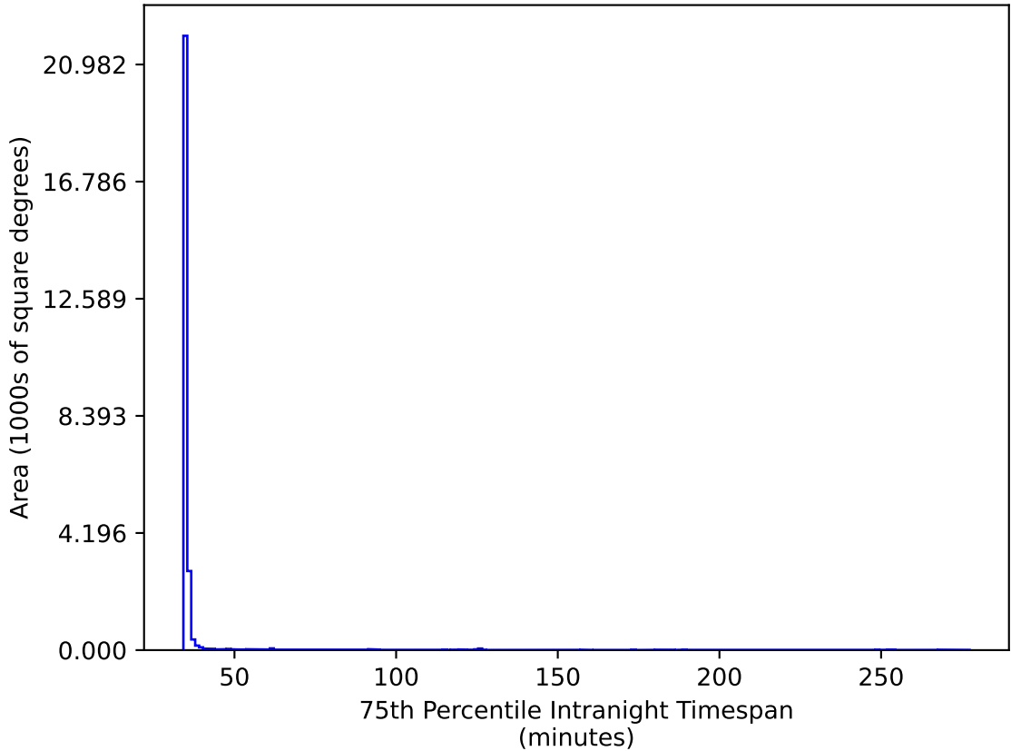
too_10_4v3.4_10yrs All sky gr bands: 75th Percentile Intranight Timespan
