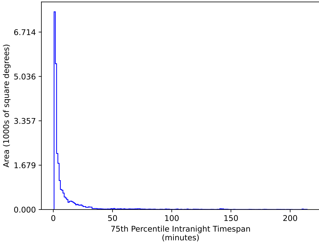
too_10_4v3.4_10yrs All sky g band: 75th Percentile Intranight Timespan
