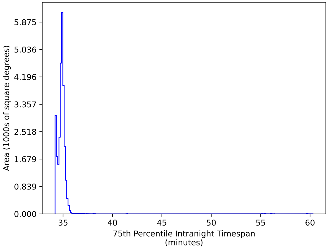
too_10_4v3.4_10yrs All sky: 75th Percentile Intranight Timespan
