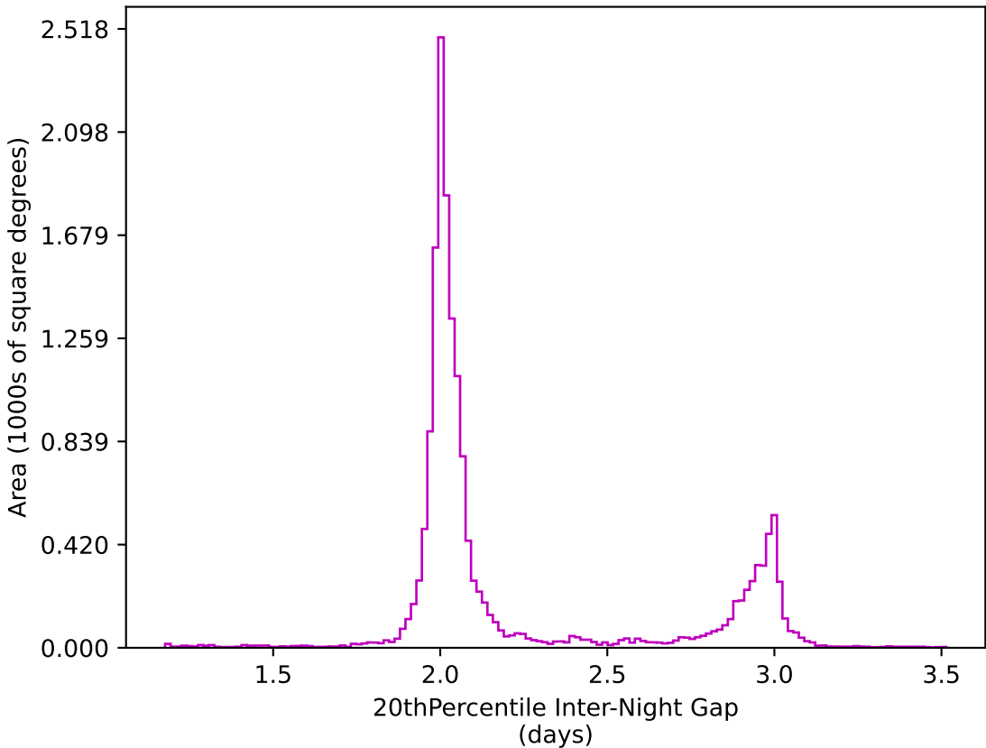
too_10_4v3.4_10yrs WFD z band: 20thPercentile Inter-Night Gap
