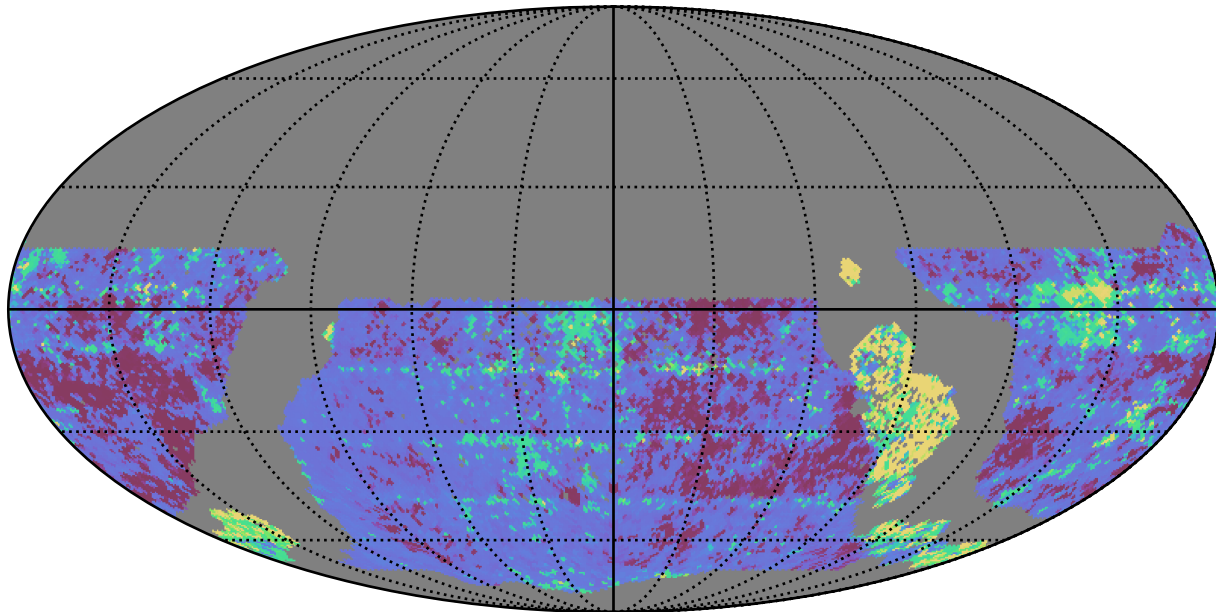
too_10_4v3.4_10yrs WFD y band: 20thPercentile Inter-Night Gap
