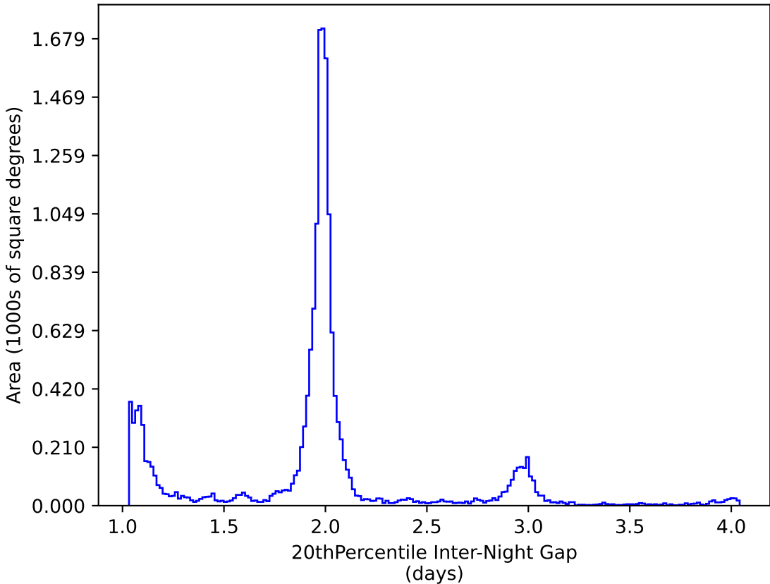
too_10_4v3.4_10yrs WFD y band: 20thPercentile Inter-Night Gap
