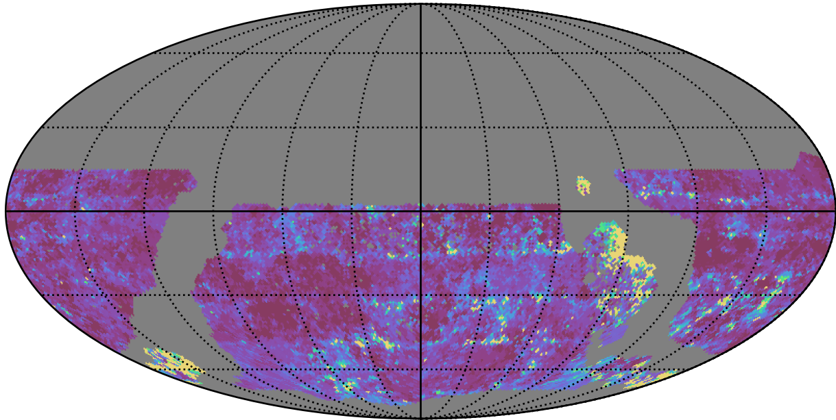
too_10_4v3.4_10yrs WFD u band: 20thPercentile Inter-Night Gap
