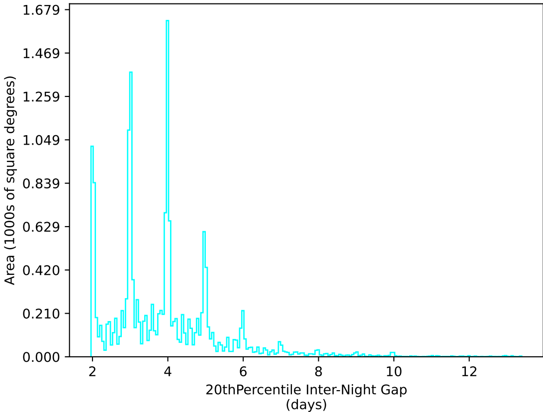
too_10_4v3.4_10yrs WFD u band: 20thPercentile Inter-Night Gap
