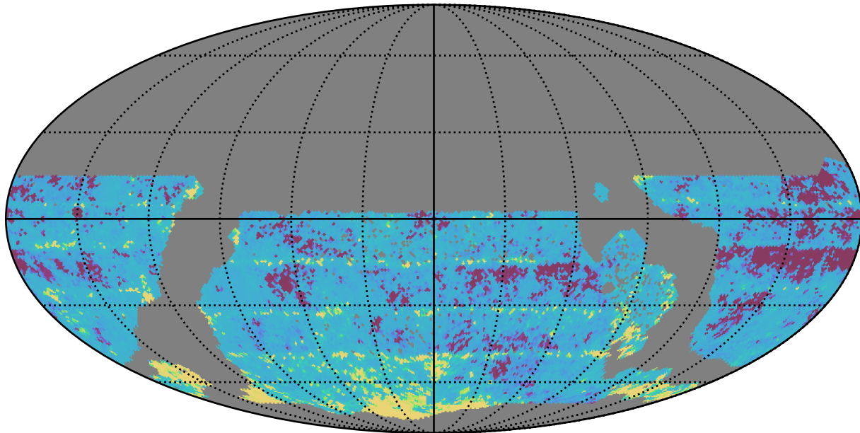
too_10_4v3.4_10yrs WFD r band: 20thPercentile Inter-Night Gap
