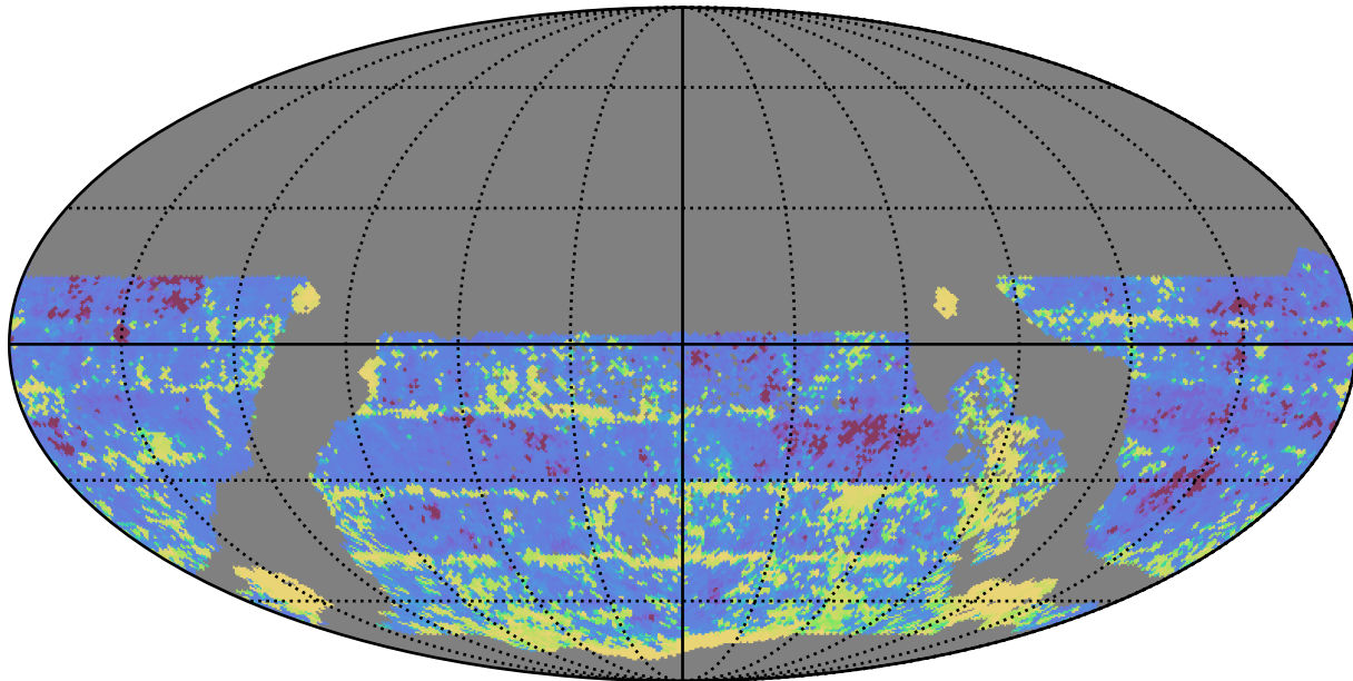
too_10_4v3.4_10yrs WFD i band: 20thPercentile Inter-Night Gap
