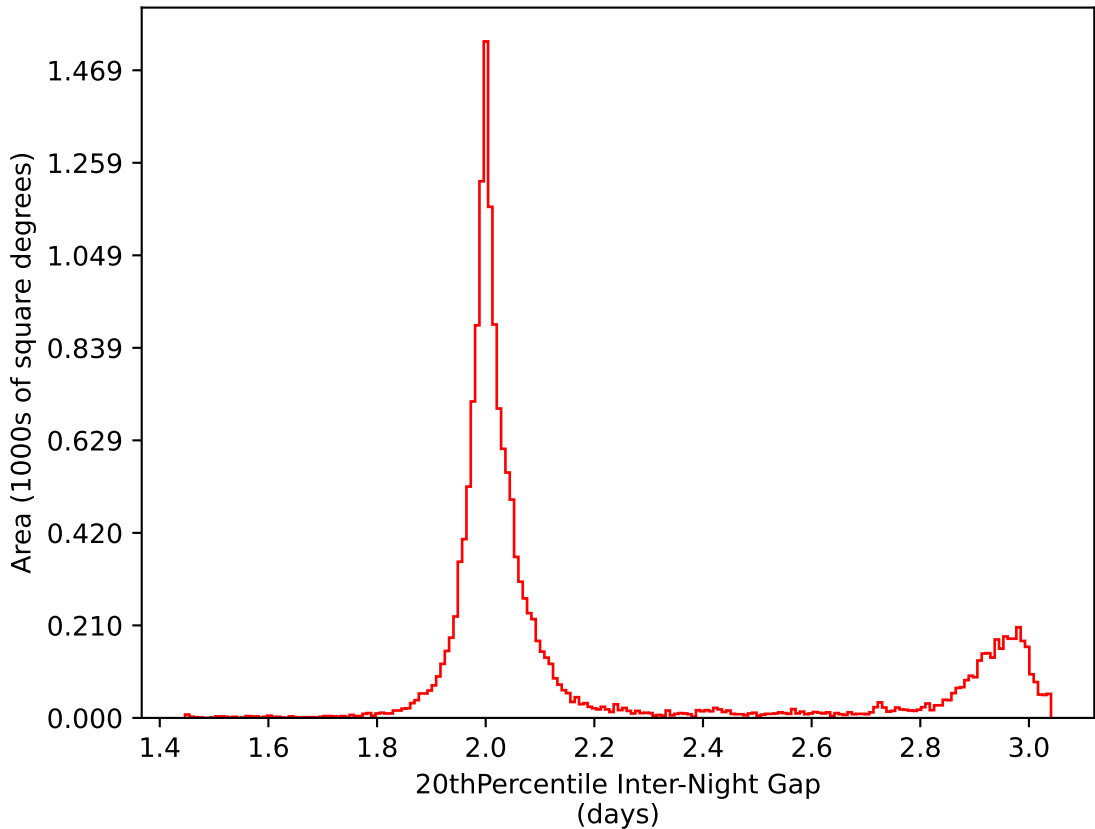
too_10_4v3.4_10yrs WFD i band: 20thPercentile Inter-Night Gap
