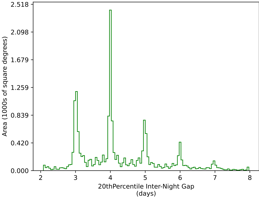
too_10_4v3.4_10yrs WFD g band: 20thPercentile Inter-Night Gap
