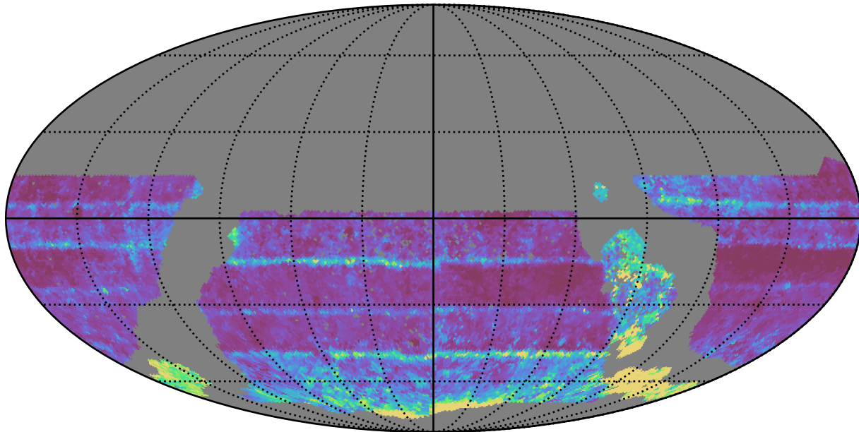
too_10_4v3.4_10yrs WFD all bands: 20thPercentile Inter-Night Gap
