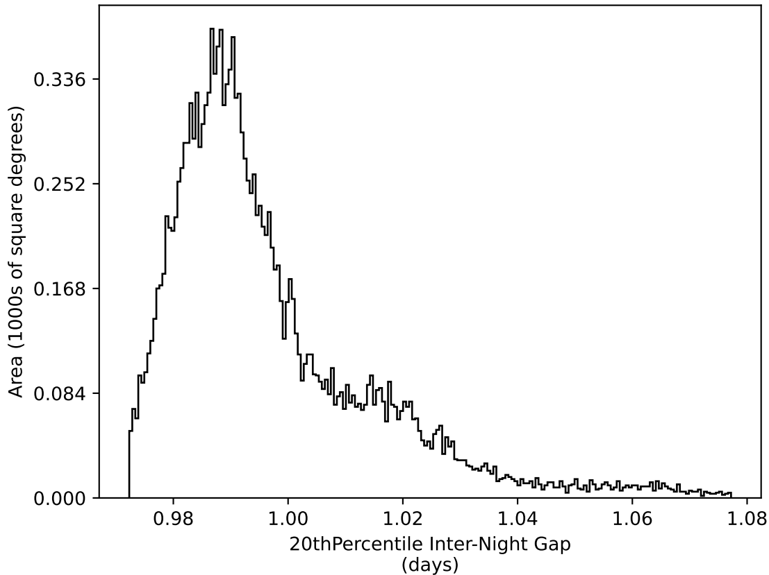
too_10_4v3.4_10yrs WFD all bands: 20thPercentile Inter-Night Gap
