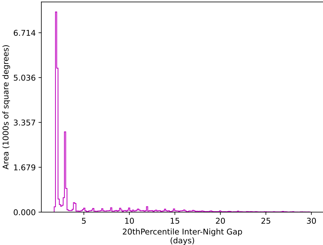
too_10_4v3.4_10yrs All sky z band: 20thPercentile Inter-Night Gap
