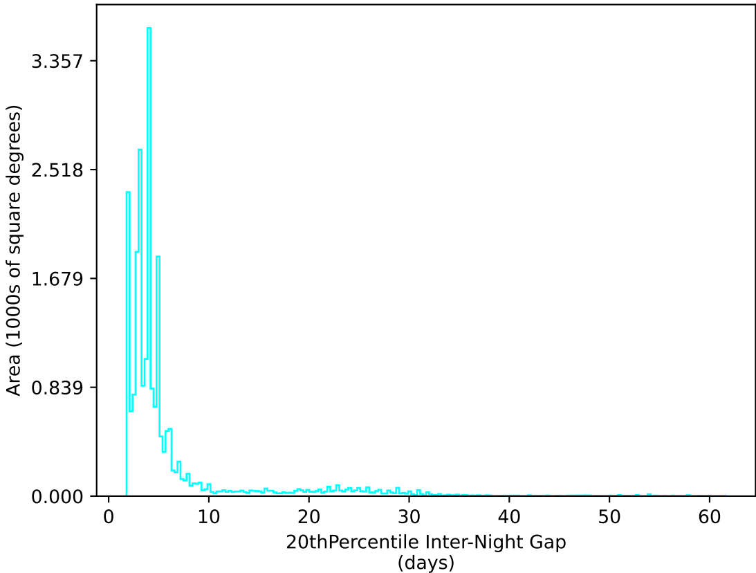
too_10_4v3.4_10yrs All sky u band: 20thPercentile Inter-Night Gap
