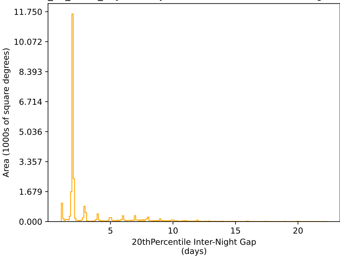
too_10_4v3.4_10yrs All sky r band: 20thPercentile Inter-Night Gap
