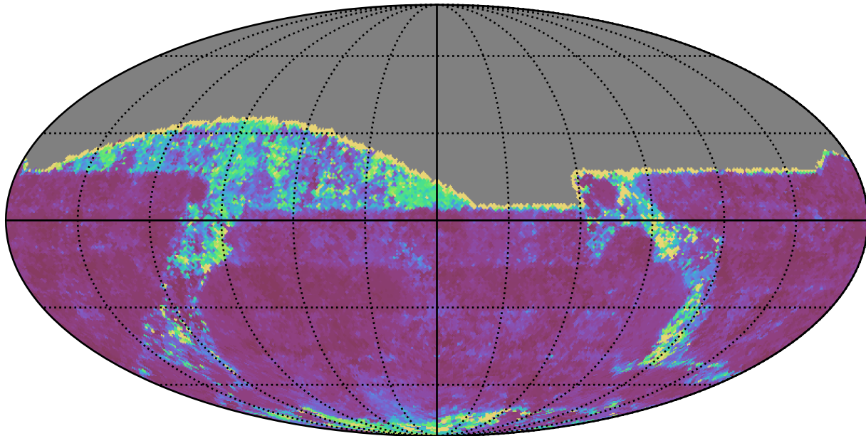
too_10_4v3.4_10yrs All sky g band: 20thPercentile Inter-Night Gap
