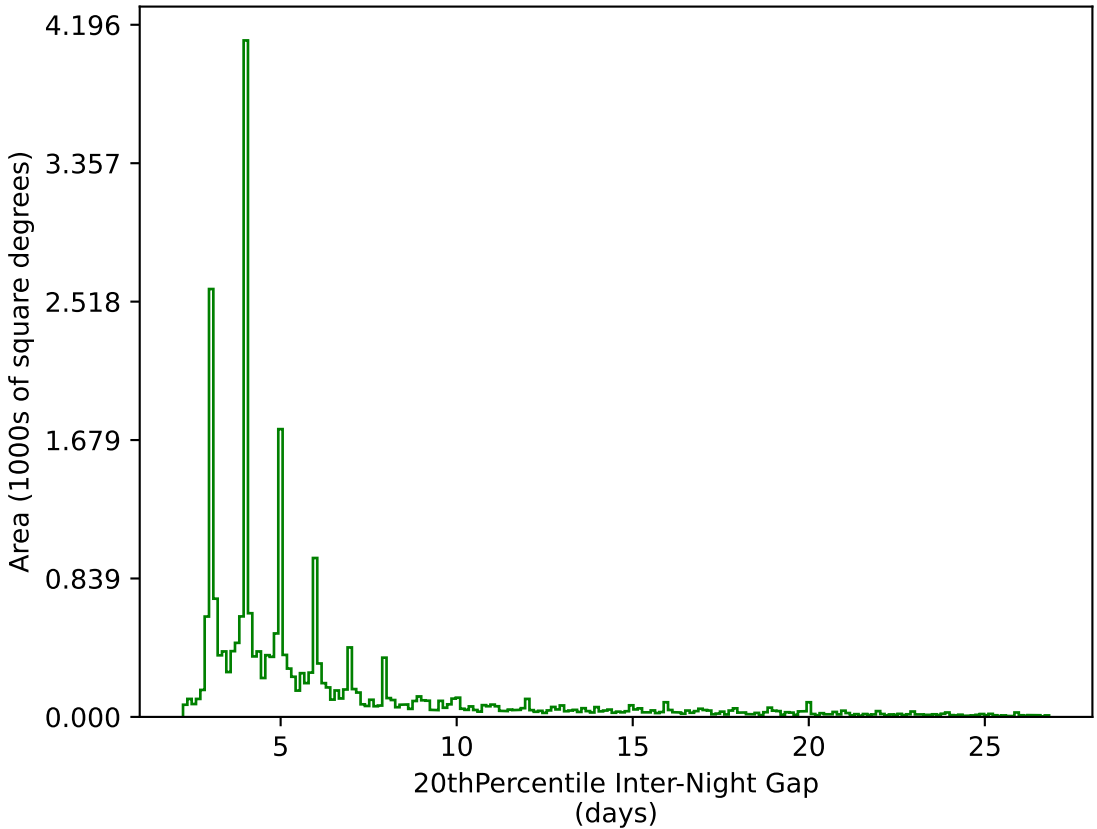
too_10_4v3.4_10yrs All sky g band: 20thPercentile Inter-Night Gap
