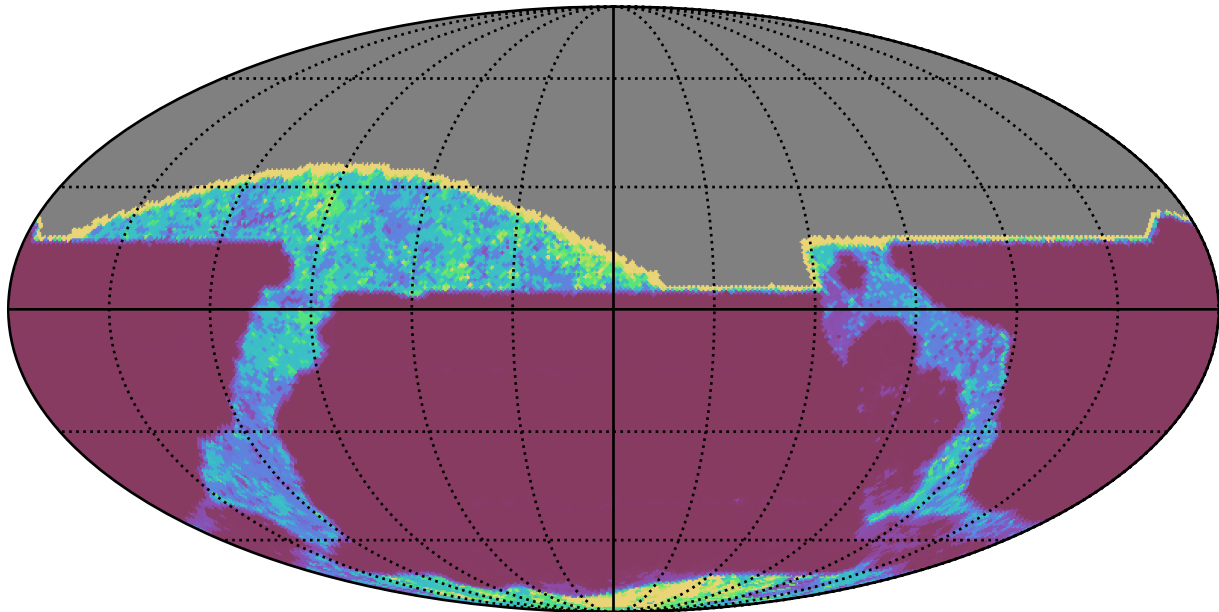
too_10_4v3.4_10yrs All sky all bands: 20thPercentile Inter-Night Gap
