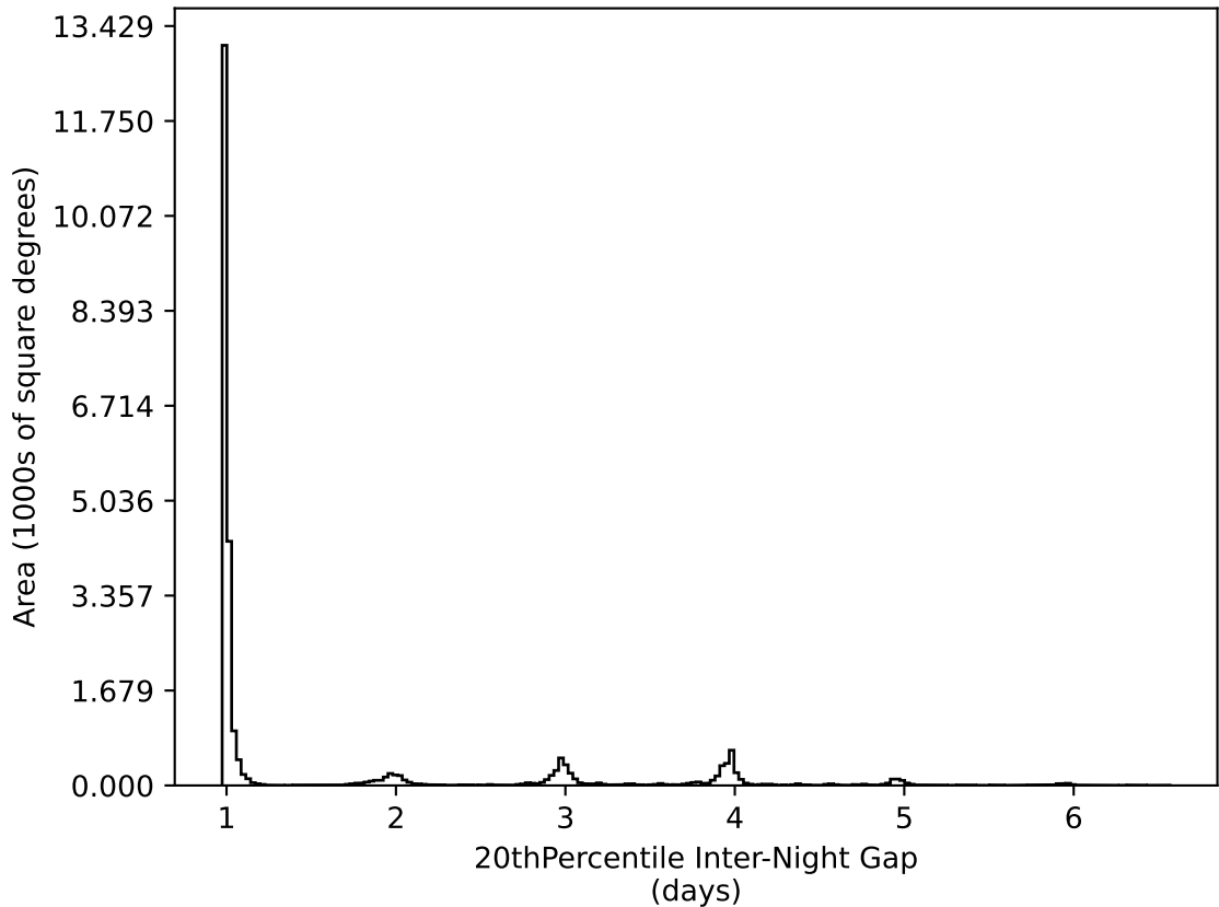
too_10_4v3.4_10yrs All sky all bands: 20thPercentile Inter-Night Gap
