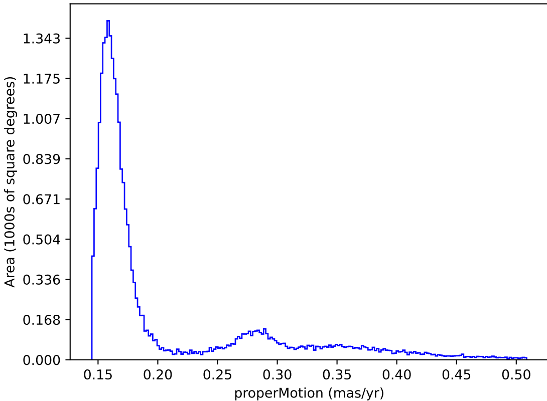
too_10_4v3.4_10yrs : properMotion
