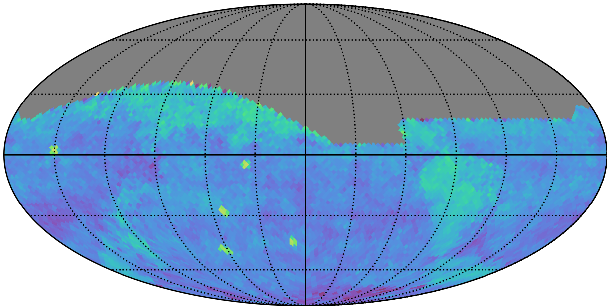
too_10_4v3.4_10yrs (g or r or i): PairFraction
